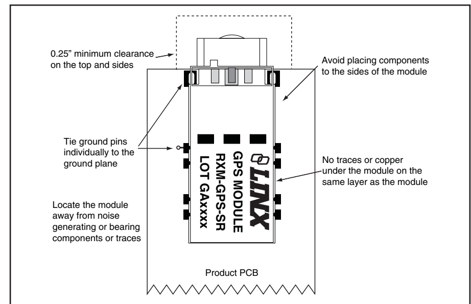
Figure 6: Antenna Considerations
